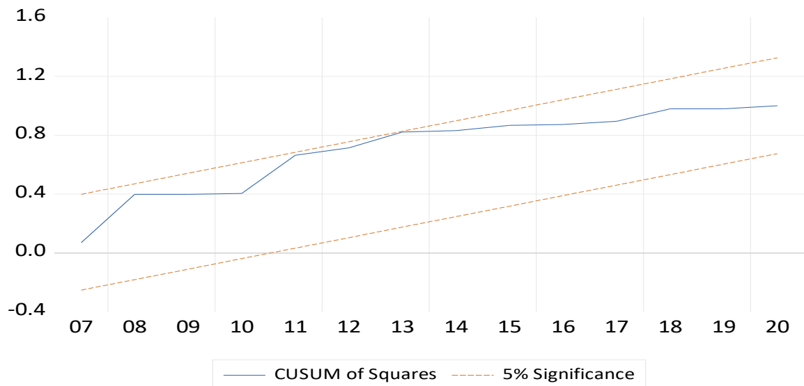
Fig. 7. CUSUMSQ test
